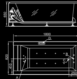
A.hydro-massage jet B.lamp C.waste D.control panel
