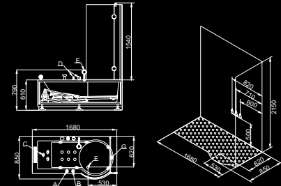
A. Electronic control panel B. Air regulator C. Hydro-massage jets D. Faucet E. Hand-held shower F. Water outlet G. Chromatherapy lighting
