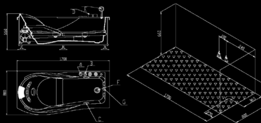
A. switch on/off B. water regulating valve C. hydromassage jet D. valve E. hand shower F. water drainage G. chromatherapy
