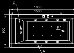
A. control panel C. hydro-massage jet D. Thermostatic faucet E. hand shower F. water outlet
